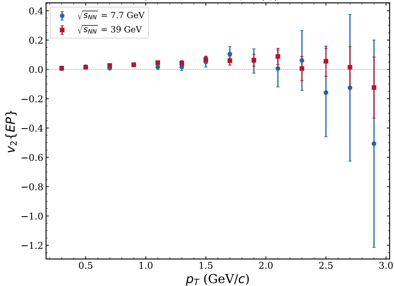
Elliptic Flow v_2 vs p_T , |\eta| < 1.0
