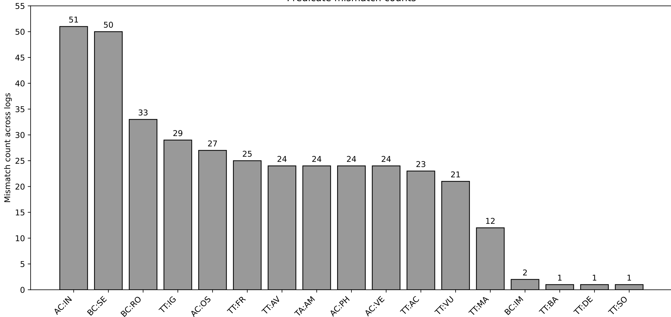
Predicate mismatch counts
