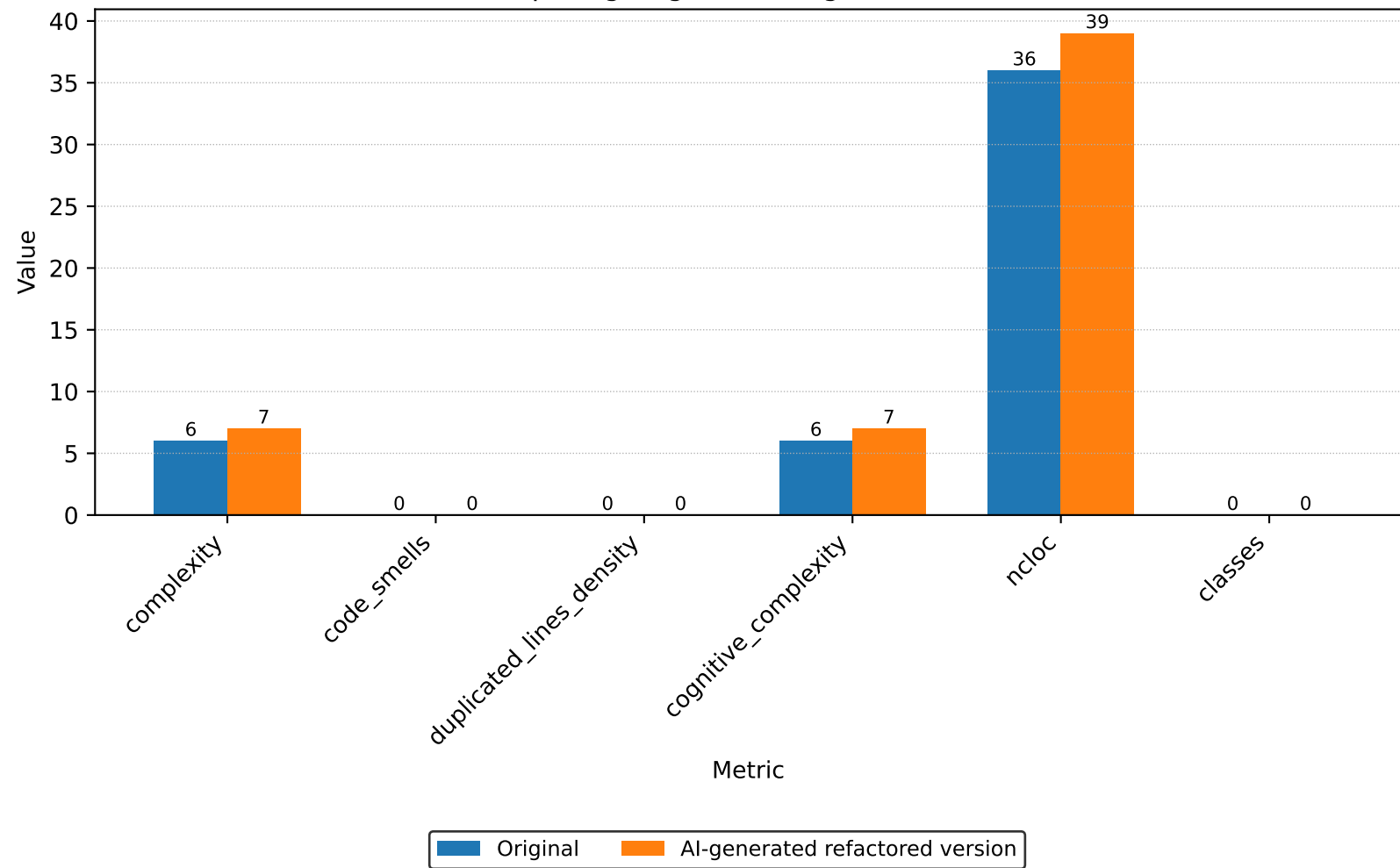
Code metrics: Comparing original vs AI-generated refactored version
