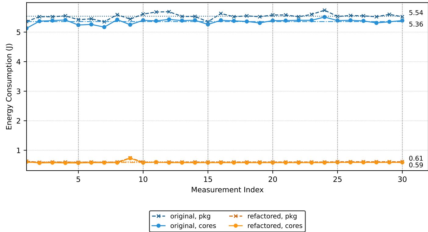
Energy consumption: Comparing original vs AI-generated refactored version
