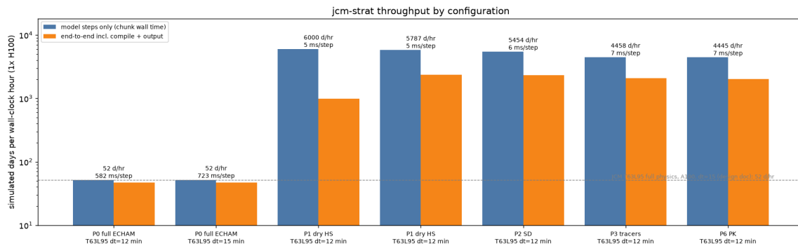
Figure 8. Simulated days per wall-clock hour on one H100. The Polvani-Kushner term adds nothing measurable to the Phase 3 cost.
