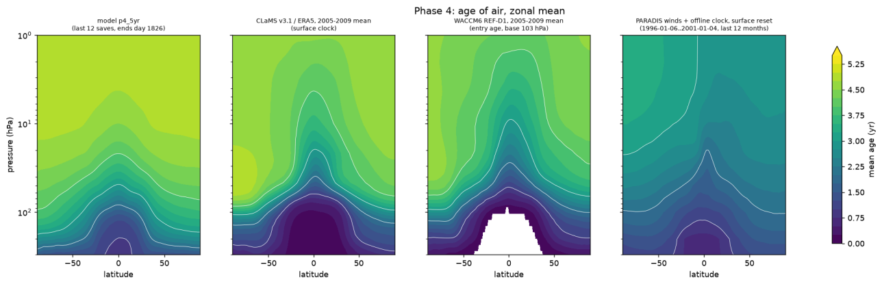
Figure 7. Zonal-mean age of air: the model (last 12 saves), CLaMS v3.1 driven by ERA5 (2005-2009 mean, a surface clock), WACCM6 REF-D1 (2005-2009 mean, an entry age relative to 103 hPa, hence younger by construction), and a surface-reset clock carried offline by the PARADIS rollout's winds for 1996-2000. The model has the right shape and the right extratropical ages but a tropical pipe that is far too old; the PARADIS-driven offline clock is too young everywhere.
