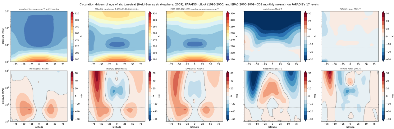
Figure 14. Zonal-mean temperature (top) and zonal wind (bottom) on PARADIS's 17 levels: the model's last year, the PARADIS rollout's 1996-2000 mean, ERA5 2005-2009 (CDS monthly means), model minus ERA5, and PARADIS minus ERA5.
