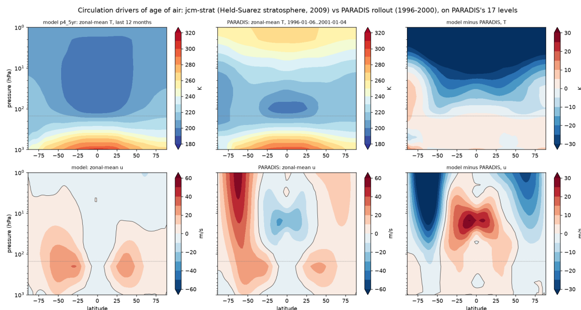
Figure 14. Zonal-mean temperature (top) and zonal wind (bottom) on PARADIS's 17 levels: the model's last year (left), the PARADIS rollout's 1996-2000 mean (middle), and model minus PARADIS (right).
