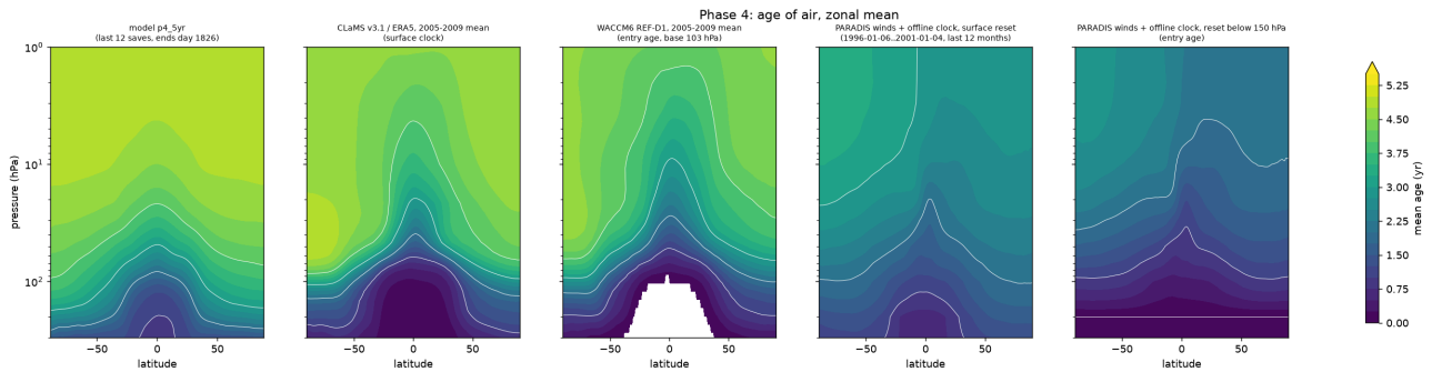
Figure 7. Zonal-mean age of air: the model (last 12 saves), CLaMS v3.1 driven by ERA5 (2005-2009 mean, a surface clock), WACCM6 REF-D1 (2005-2009 mean, an entry age relative to 103 hPa, hence younger by construction), and two clocks carried offline by the PARADIS rollout's winds for 1996-2000 (surface reset; reset below 150 hPa). The model has the right shape and the right extratropical ages but a tropical pipe that is far too old; the PARADIS-driven offline clocks are too young everywhere.
