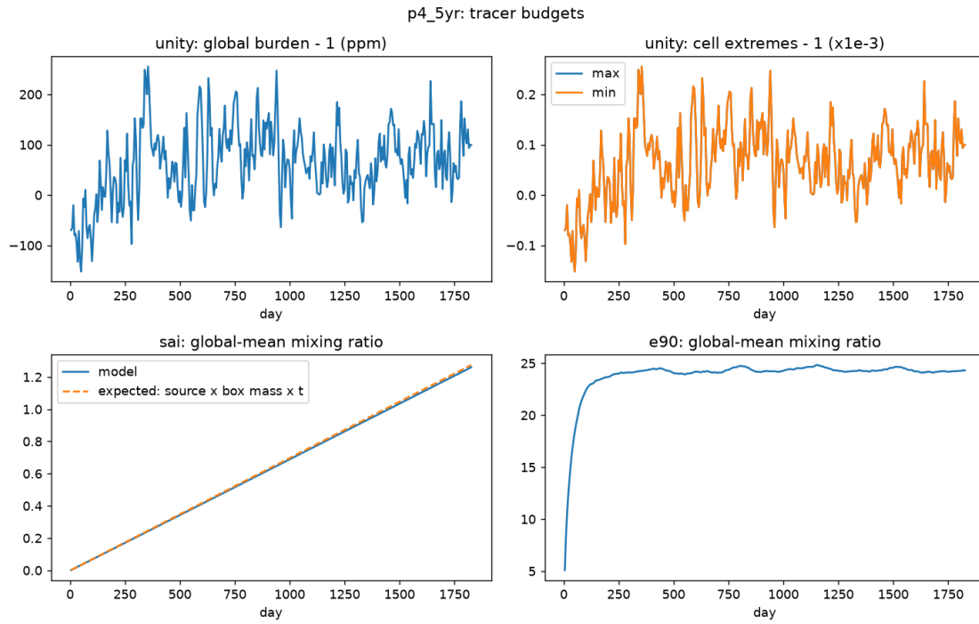
Figure 11. Five-year tracer budgets: unity's burden and cell extremes stay within 3\text{e-}4 of one throughout; the sai burden follows the analytic source line for five years; e90 stays saturated.
