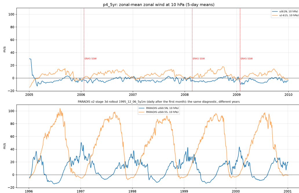
Figure 9. Zonal-mean zonal wind at 10 hPa and 61N (blue) and 61S (orange). Top: the model, 5-day means, with the ERA5 sudden-warming dates marked; there is no winter westerly jet to disrupt in either hemisphere. Bottom: the same diagnostic in the PARADIS rollout for 1996-2000 (daily): both polar-night jets present, no reversal in five winters, the northern winter jet weakening from 31 to 16 m/s over the rollout.
