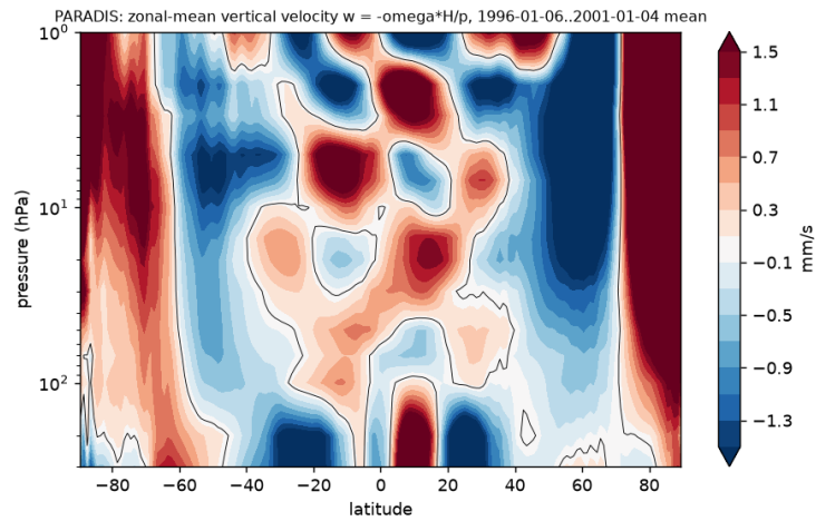
Figure 15. PARADIS zonal-mean vertical velocity, w = -\omega H/p , 1996-2000 mean. Checkerboard above 10 hPa and polar ascent are not physical; the tropical column changes sign between 100 and 50 hPa.
