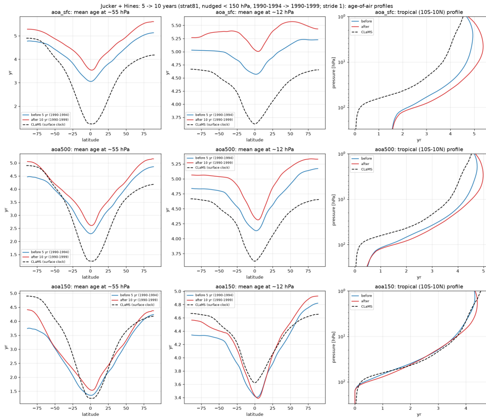
Figure 9. Age of air after five (blue) and ten (red) years, CLAMS dashed: surface clock, 500 hPa clock and entry-age clock (rows). The entry-age clock moves 0.1-0.2 yr at 55 hPa (0.6 over the Antarctic) and is converged at 12 hPa in the tropics; the two lower clocks rise 0.3-0.5 yr everywhere.
