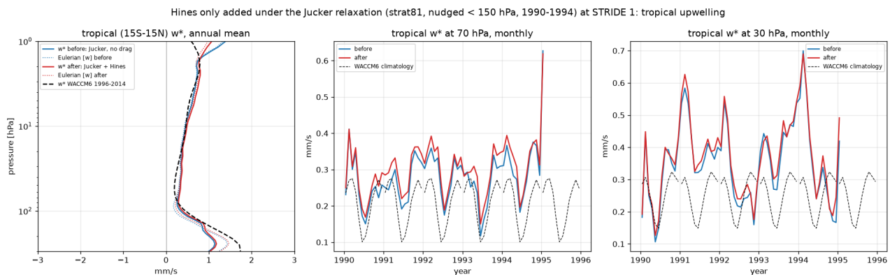
Figure 8. The Phase 13d pair at stride 1: annual tropical w^* (WACCM6 dashed) and monthly w^* at 70 and 30 hPa. The model sits above WACCM6's cycle in most months with the seasonal phase right; compare Figure 3, the same runs from the 06 UTC frames.
