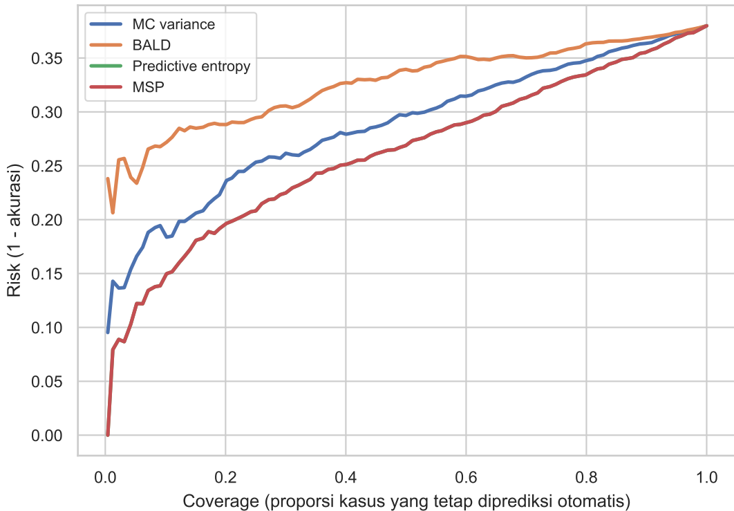
Kurva Risk-Coverage — makin rendah makin baik
