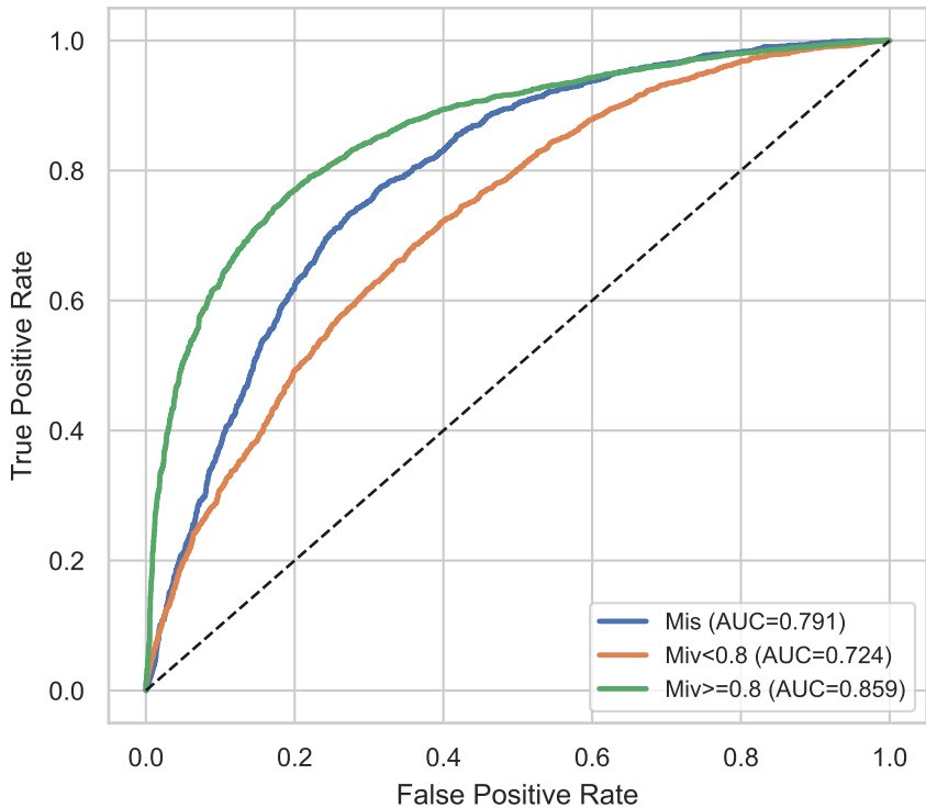
Skenario A — ROC one-vs-rest
