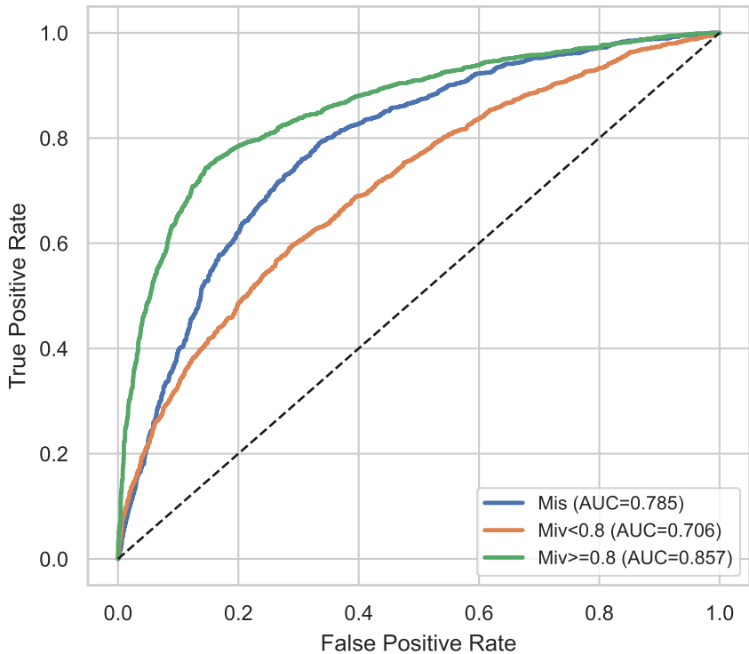
Skenario B — ROC one-vs-rest
