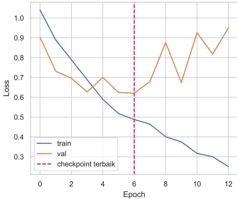
Flat multiclass fold 1
