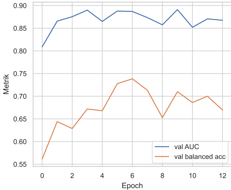
Flat multiclass fold 1
