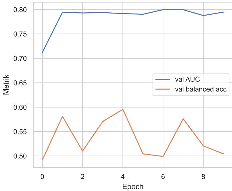
Flat multiclass fold 2
