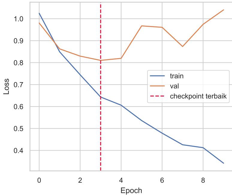
Flat multiclass fold 2
