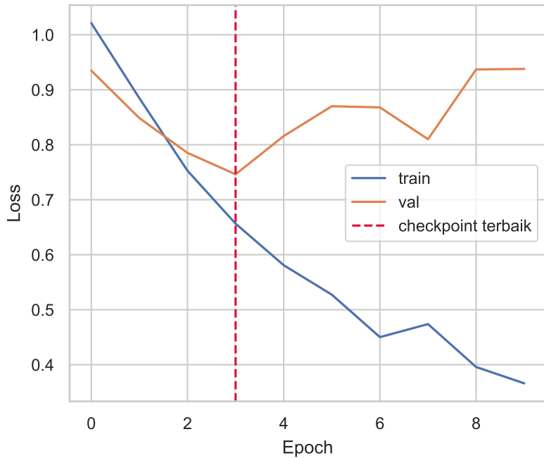
Flat multiclass fold 4
