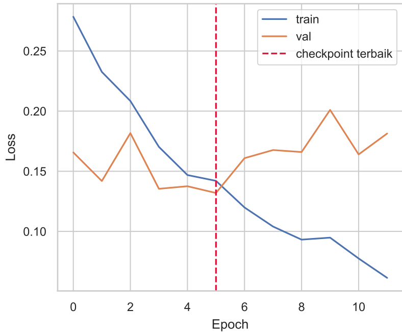
Stage 1 fold 0 seed 46
