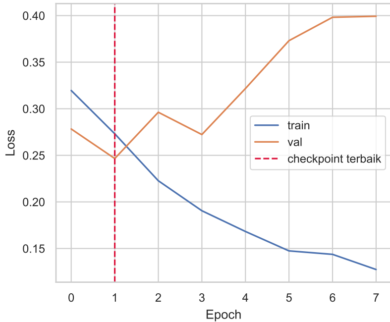
Stage 1 fold 1 seed 43
