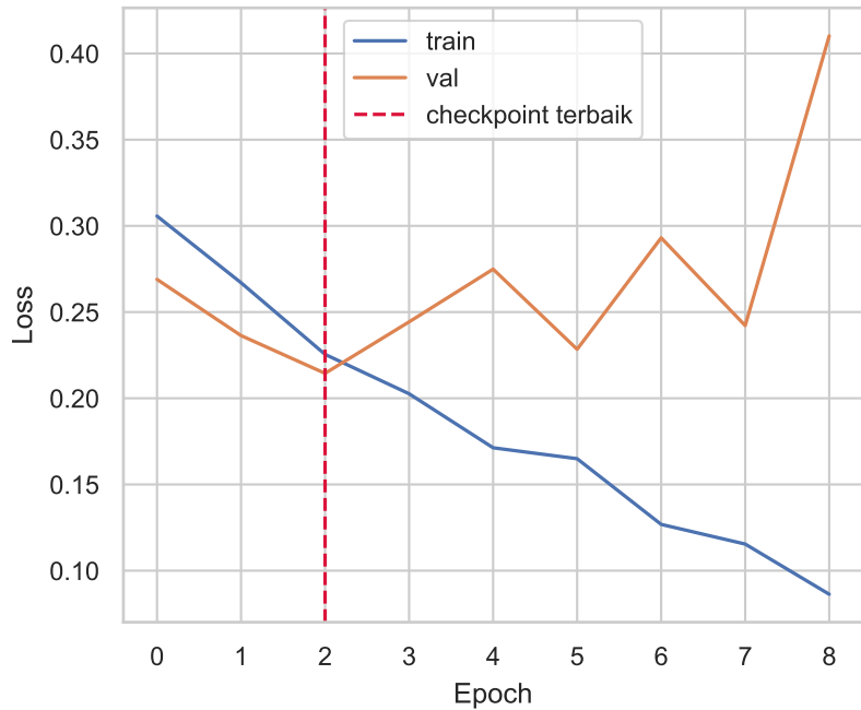
Stage 1 fold 2 seed 44
