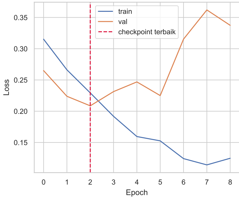
Stage 1 fold 3 seed 43
