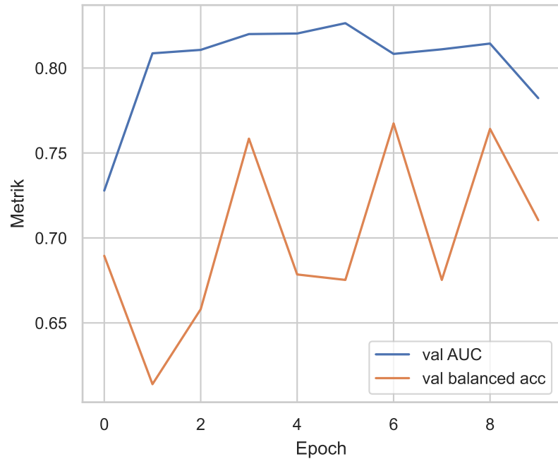
Stage 1 fold 3 seed 45
