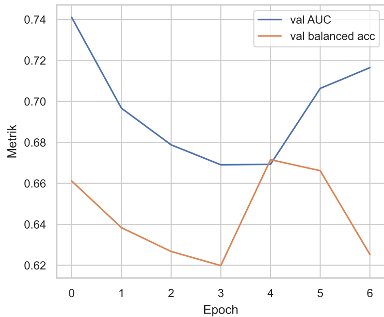
Stage 1 fold 4 seed 45
