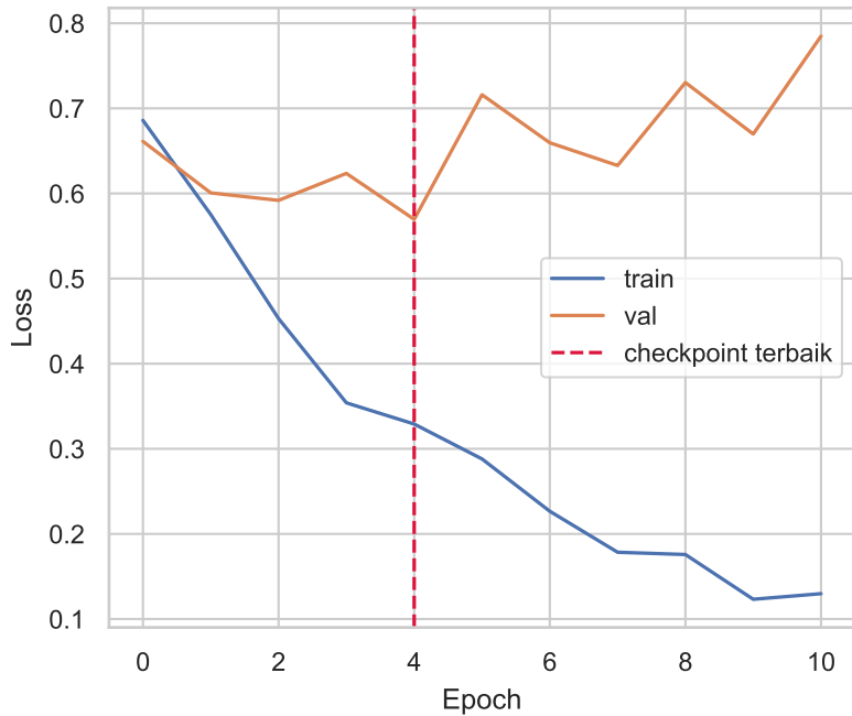
Stage 2 (gt) fold 1
