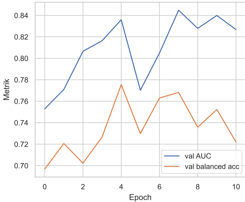
Stage 2 (gt) fold 1
