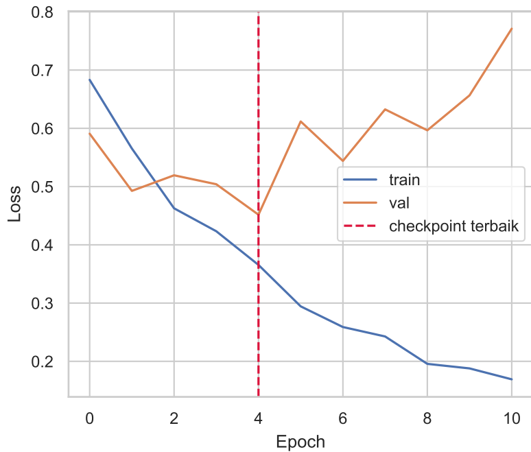
Stage 2 (gt) fold 2
