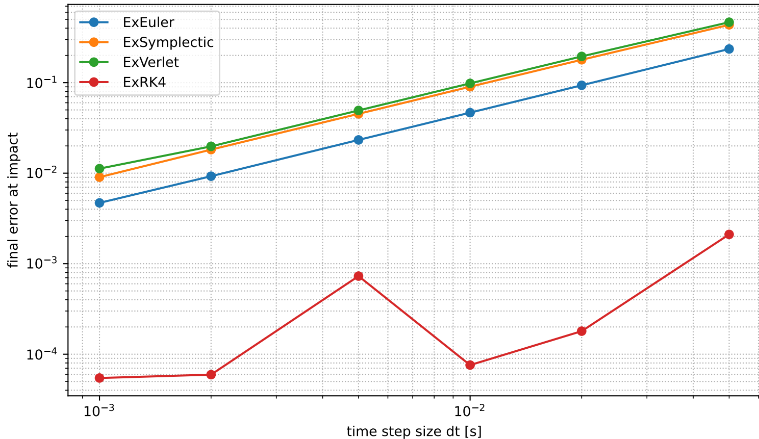
Final Error at Impact vs dt (per method)
