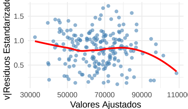
Scale-Location Plot
