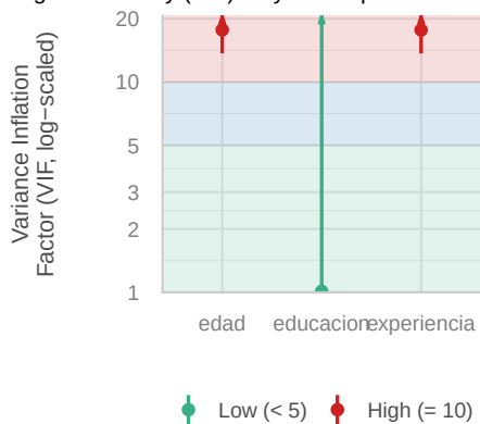
Collinearity
