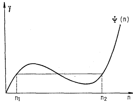
Fig. 4. Maxwellian construction of the coexistence value \gamma
