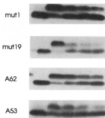
FIG. 3. Stability of the electrophoretic mobility shift of cAR1 mutants. Cells expressing wild-type or mutant cAR1s were incubated with cAMP ( 10^{-5} M, 15 min) washed four times with ice-cold PB, resuspended to 5 \times 10^7 /ml, and incubated on ice for the indicated times. Aliquots of cells were transferred to sample buffer before the addition of cAMP (-), following the 15 min stimulation and at 20, 60, and 120 min after the initiation of the third PB wash. (See "Materials and Methods" for explanation of time scale.) Cluster 1 mutants are defined in Table I. A62 and A53 are third intracellular loop mutants (16). The data shown are representative of at least two independent experiments.
