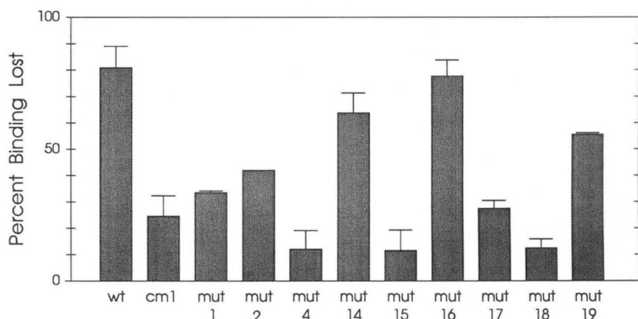
FIG. 2. Loss of ligand binding by cAR1 mutants. Cells expressing wild-type (wt) or mutant cAR1s were incubated without or with cAMP ( 10^{-5} M, 15 min), washed, resuspended to 10^8 /ml, and analyzed for LLB by the sedimentation assay described under "Materials and Methods." Plotted for each cell line is the percentage of binding exhibited by untreated cells which is lost upon cAMP pretreatment. Values represent the means \pm range of triplicate determinations from two independent experiments. mut2 was analyzed in only one experiment.
