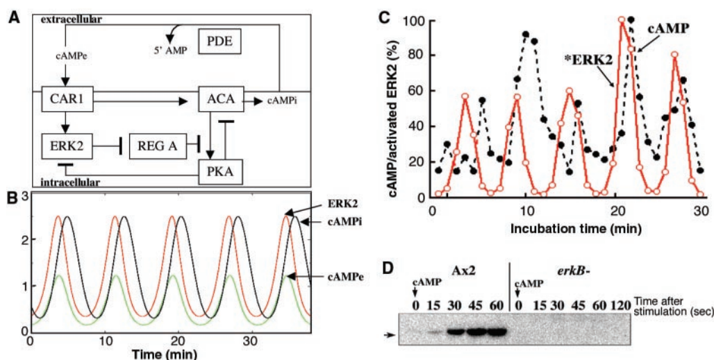
Fig. 2. Spontaneous oscillations. (A) The circuit that generates oscillations is modified from Laub and Loomis (13). Arrows indicate activation; bars indicate inhibition. PDE is the secreted phosphodiesterase that hydrolyzes extracellular cAMP (cAMPe). CAR1 is the cAMP receptor; ACA is the aggregation adenylyl cyclase; PKA is the cAMP-dependent protein kinase; ERK2 is the MAP kinase; and RegA is the phosphodiesterase that hydrolyzes internal cAMP (cAMPi). Connecting intermediates, such as trimeric G protein, phosphatidylinositol 3-kinase, CRAC, and Pianissimo, are not included in the present analyses, and the proposed interactions need not be direct. (B) Output of the circuit simulation of cells at 4 hours of development. Periodic changes in ERK2 activity and the internal and external levels of cAMP are indicated (arbitrary units). (C) Measured changes in phospho-ERK2 and cAMP in pulse-developed cells that were washed and resuspended at 5 \times 10^7 cells/ml. Samples were taken at 1-min intervals. The NIH Image package was used to quantify the level of phospho-ERK. Results are representative of three inde-
