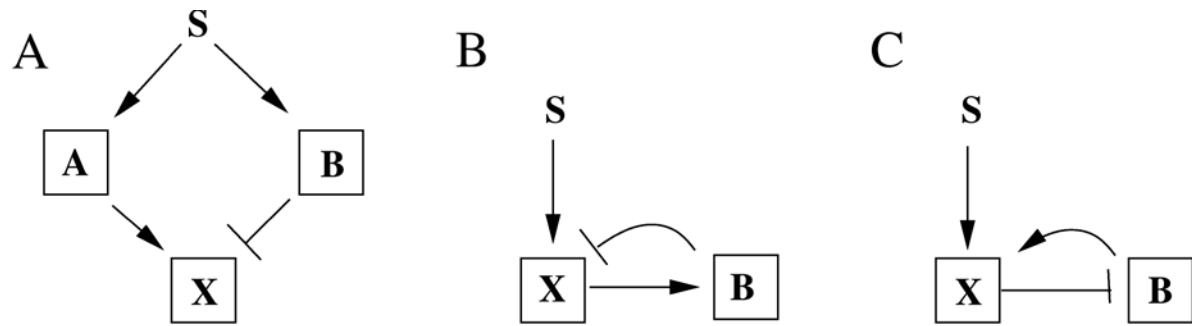
Fig. S8. Core model topologies.
