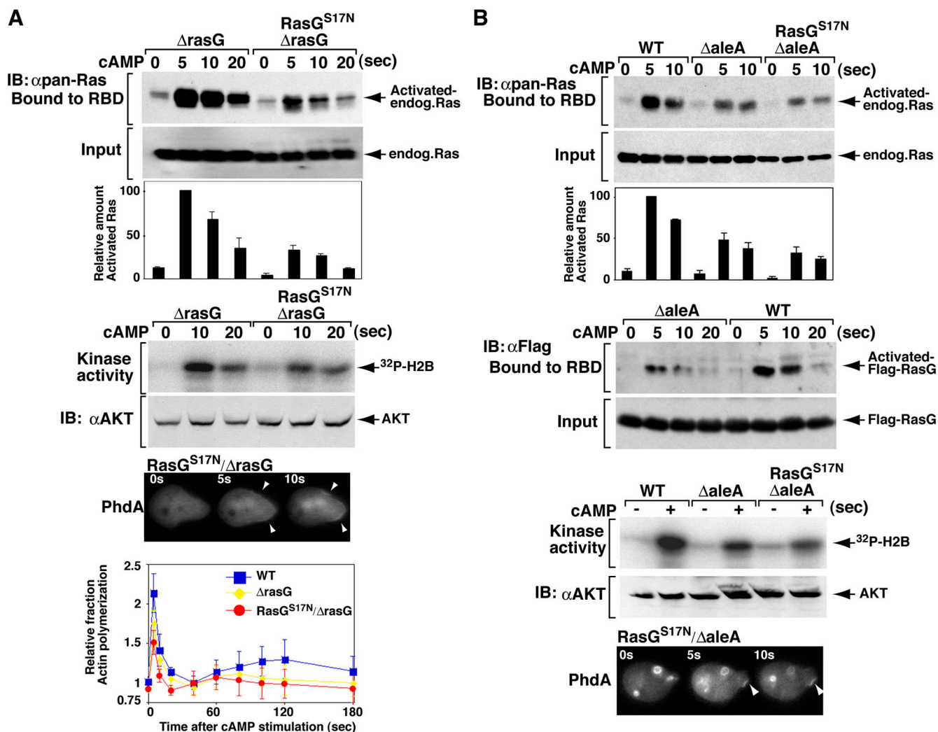
Figure 7. Activation of Akt/PKB and Ras. The effects of \text{RasG}^{\text{S17N}} on Akt/PKB, Ras activation, and production of \text{PI}(3,4,5)\text{P}_3 in rasG (A) and aleA (B) null cells were assayed as described in the legends to Figs. 1–4. The results were similar in five independent assays.
