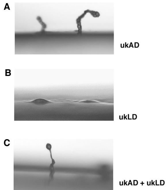
FIG. 6. Complementation of the PDE-null aggregate-less phenotype. (A) The phenotype of uk7 cells overexpressing pdsA \Delta AR from the aggregation promoter. (B) The phenotype when expression is from the vegetative/late promoters. If the two transformants are mixed in a 1:1 ratio, morphologically normal fruiting bodies are restored (C).
