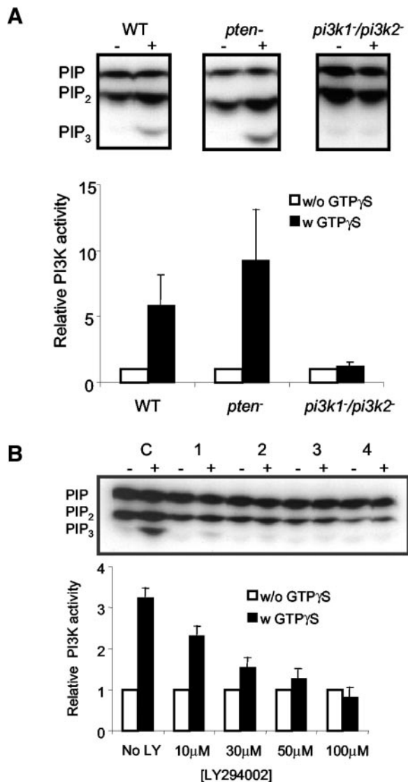
Figure 4. Activation of PI3K in response to GTPγS in various cell lines and the effect of LY294002 on PI3K activation. (A) PI3K activation of wild-type, pten - and pi3k1 - / pi3k2 - cells. The cell lysates of these three different cell lines were treated with GTPγS, and the cell lysates were incubated with ATPγ 32 P for 3 min. The lipids were extracted and were analyzed by TLC plate. Image J was used to measure the intensities of the PI(3,4,5)P 3 bands. The data of activated level (w GTPγS) were normalized to the basal level (w/o GTPγS). The graph represents the average of three independent experiments. (B) The effect of different concentrations of LY294002 on PI3K activation in wild-type cells. Wild-type cell lysates were either incubated with no LY294002 (C) or with 10, 30, 50, and 100 μM of LY294002, respectively (1–4), in the presence or absence of GTPγS. The graph represents the average of two independent experiments
