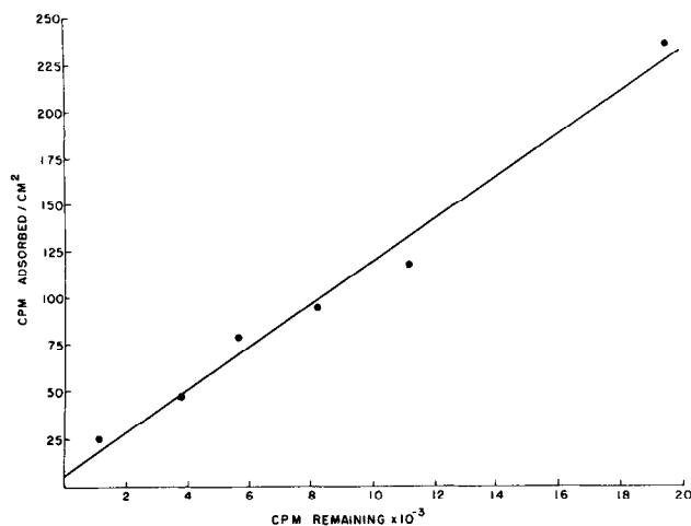
FIG. 2 (left). Adsorption isotherm for [ 3 H]cAMP in diffusion chamber. The data points represent the results of experiments in which 1,965, 3,746, 8,222, 11,137, 15,596, and 27,326 cpm of [ 3 H]cAMP were added to the chamber. Specific activity was 16 Ci/mmol.
