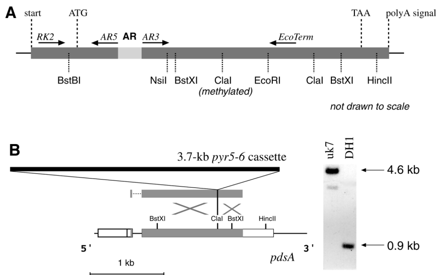
FIG. 1. Strategy used in inactivating pdsA . (A) The structure of the gene with relevant restriction sites and primers. All Southern blots employed genomic DNA digested with BstXI and were probed with a 0.9-kb BstXI fragment that contains most of the pdsA coding sequence. As expected, a 0.9-kb band is detected in parental DNA digested with BstXI . (B) Disruption in the uk7 strain (uracil selection). See Materials and Methods for details of constructs.
