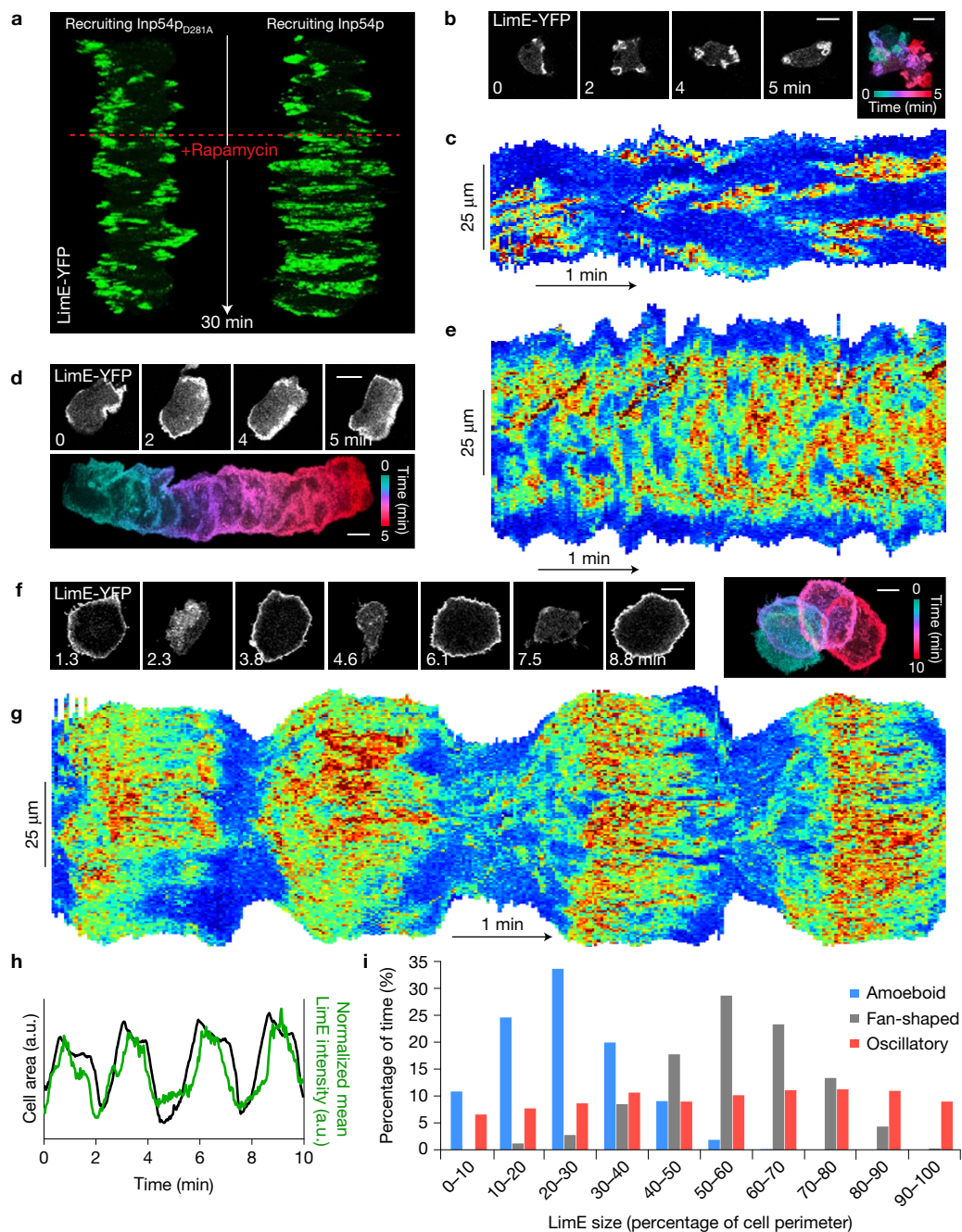
Figure 2 Actin profiles show distinct spatiotemporal patterns in amoeboid, fan-shaped and oscillatory cells. (a) T-stacks of LimE \Delta coil-YFP (LimE) in initially amoeboid cells before and after recruiting inactive (left) or active (right) Inp54p. The red dashed line indicates the addition of rapamycin. (b–g) Time-lapse confocal images and colour-coded overlays of the YFP fluorescence intensities at 2s intervals of an amoeboid (b), fan-shaped (d) and oscillatory cell (f) expressing LimE. Scale bars represent 10 \mu m. Kymographs of cortical LimE intensity in the same amoeboid (c), fan-shaped (e) and oscillatory cells (g). Durations of the
