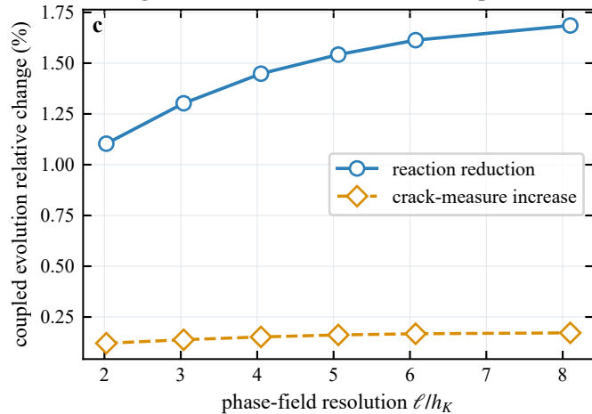
Damage evolution adds a smaller mesh-dependent shift
