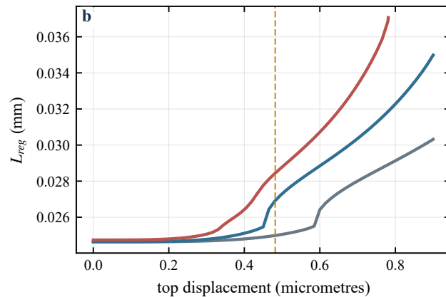
Regularized crack evolution
