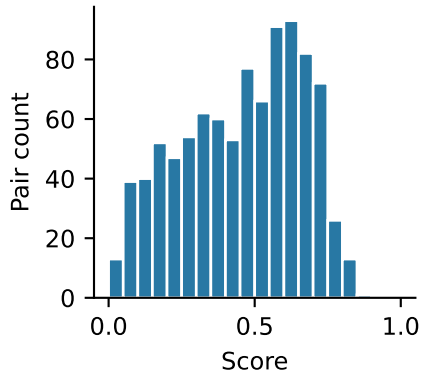
Overlapping-pair IoU
