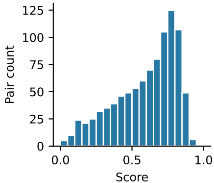
Overlapping-pair Dice
