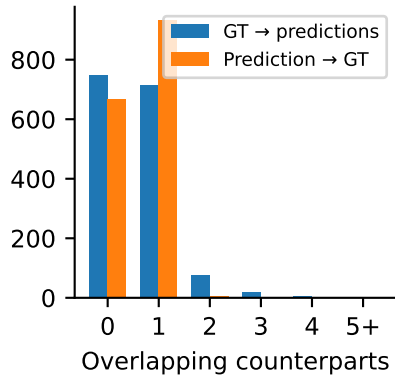
Fragmentation / merging
