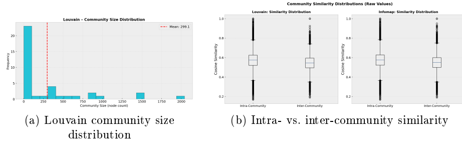
Fig. 2. Community diagnostics for Custom-WikiCS. The cleaned graph contains non-trivial communities, and those communities remain semantically coherent
