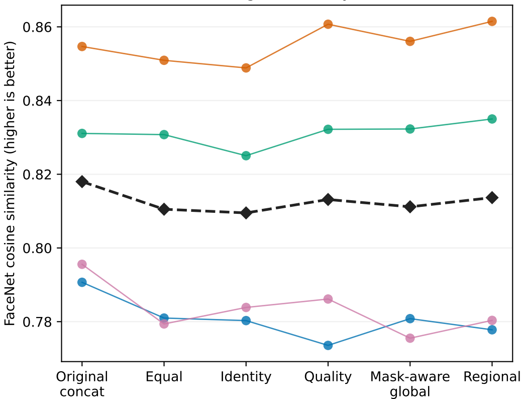
Target similarity
