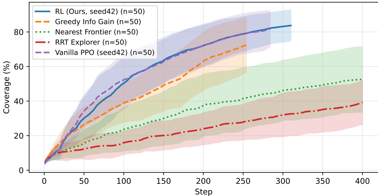
Coverage over episode (mean \pm std across eval episodes)
