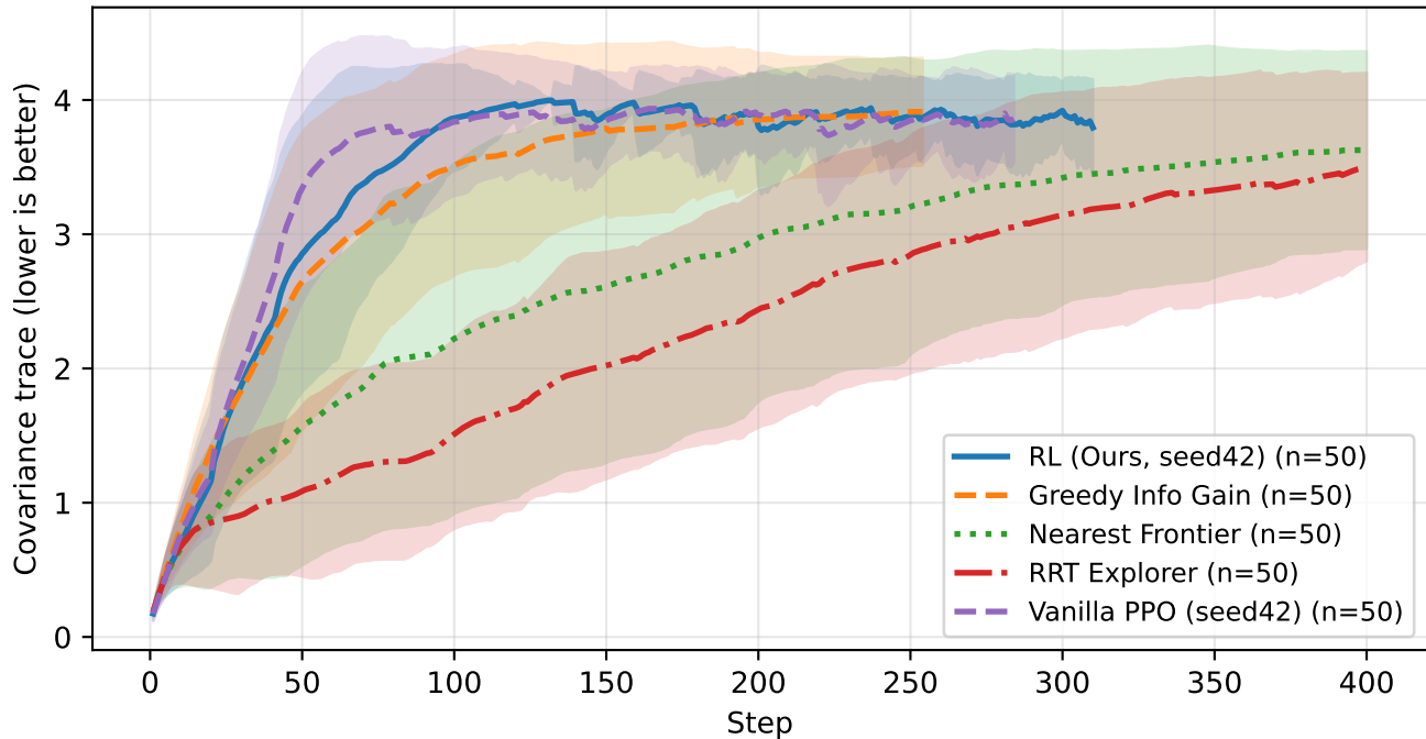
Covariance trace over episode (mean \pm std across eval episodes)
