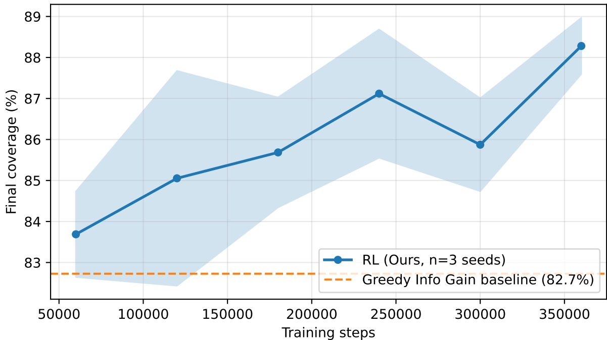
RL learning curve: coverage
