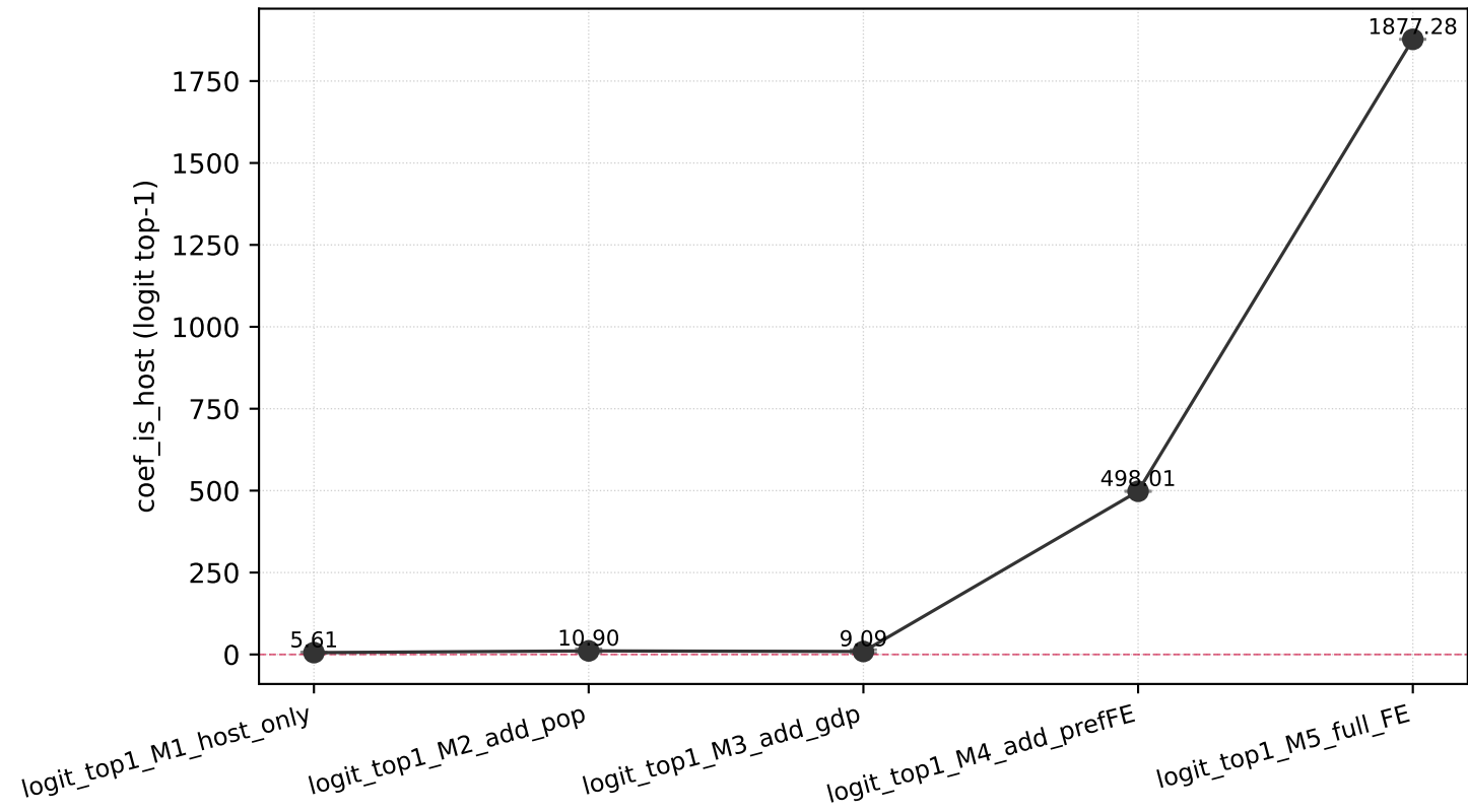
Csurilla-type confounder attenuation (2012-2022 tennou)
