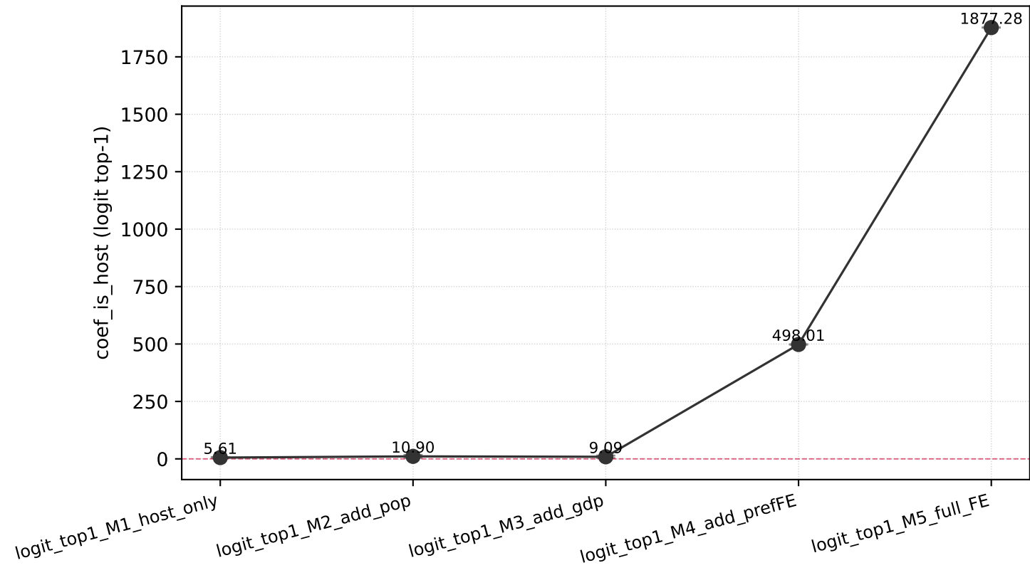
Csurilla-type confounder attenuation (2012-2022 tennou)
