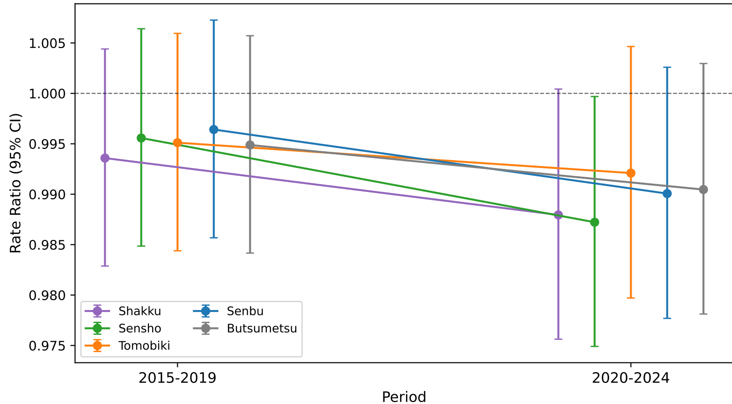
Figure 4: Temporal Trend of Rokuyo Effect on Daily Births (ref: Taian, 5-year blocks)
