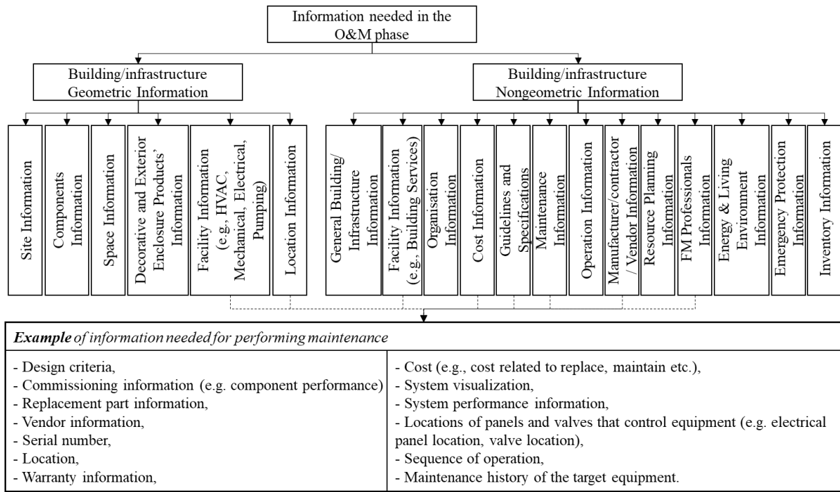
Figure 2 Information requirements in O&M phases [3,33,34,35,36,37,38] Although a large amount of effort has been made in achieving smart O&M management, a lack of well-organised framework/system to link all assets efficiently, as well as the capability to manage required information, is one of the key problems in O&M management.
