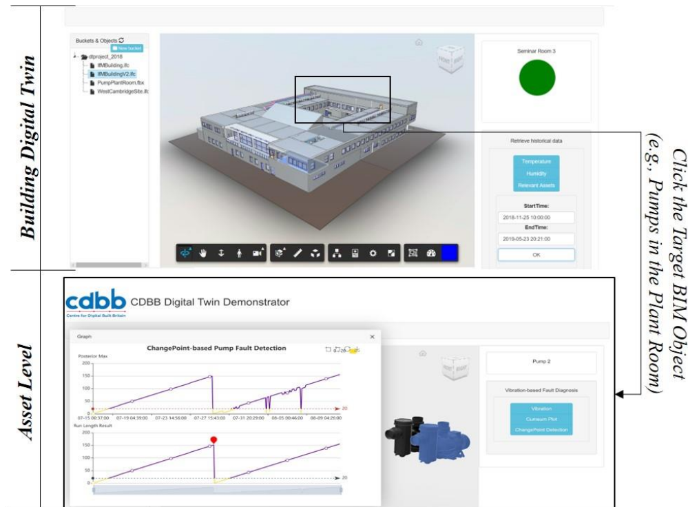
Figure 18 Asset Monitoring service provided by DT platform
