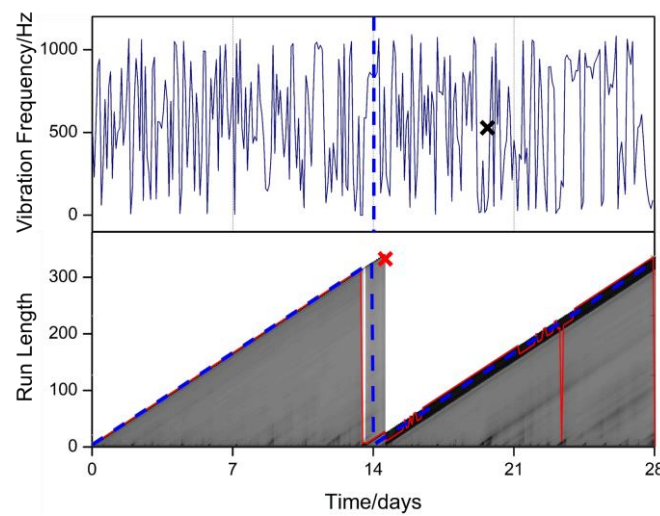
Figure 17 Detection of the pump anomalous event by BOCPD procedure
