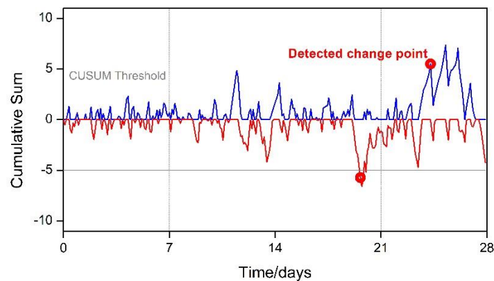
Figure 16 Detection of the pump anomalous event by CUSUM procedure
