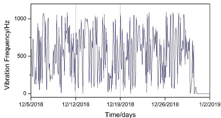
Figure 12 Vibration frequency sequence in the pump shutdown scenario
