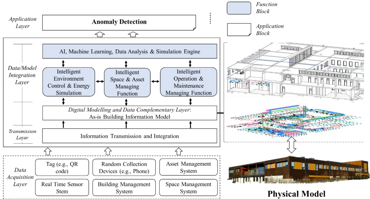
Figure 9 The developed building DT (modified from [44] and [64])
