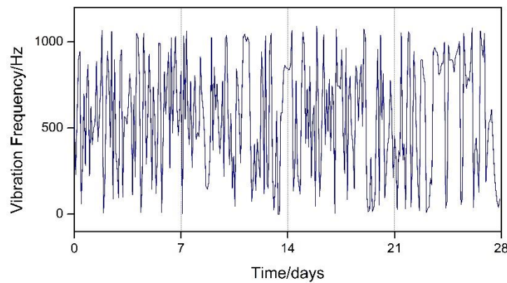
Figure 15 Vibration frequency sequence in the pump anomalous scenario
