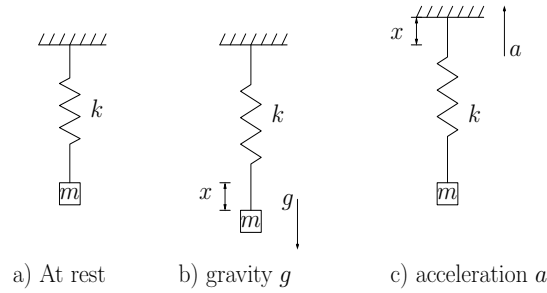
Figure 3.1. Spring-mass accelerometer.
