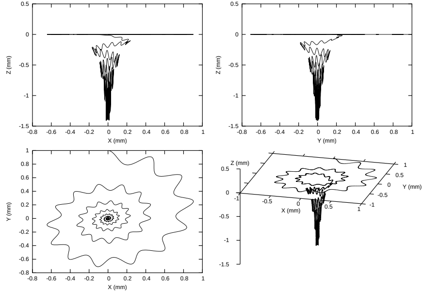
Figure 4.3. Projections of simulated particle trajectory.
