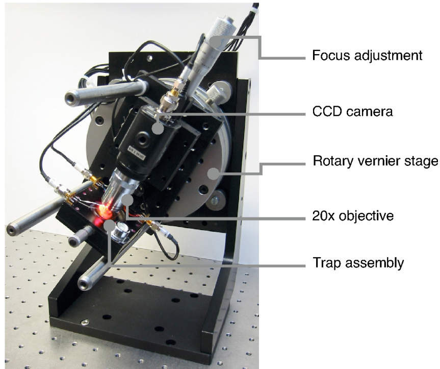
Figure 4.14. Experimental apparatus for characterization by video microscopy.
