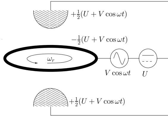
Figure 3.3. 3D Paul trap (schematic).
