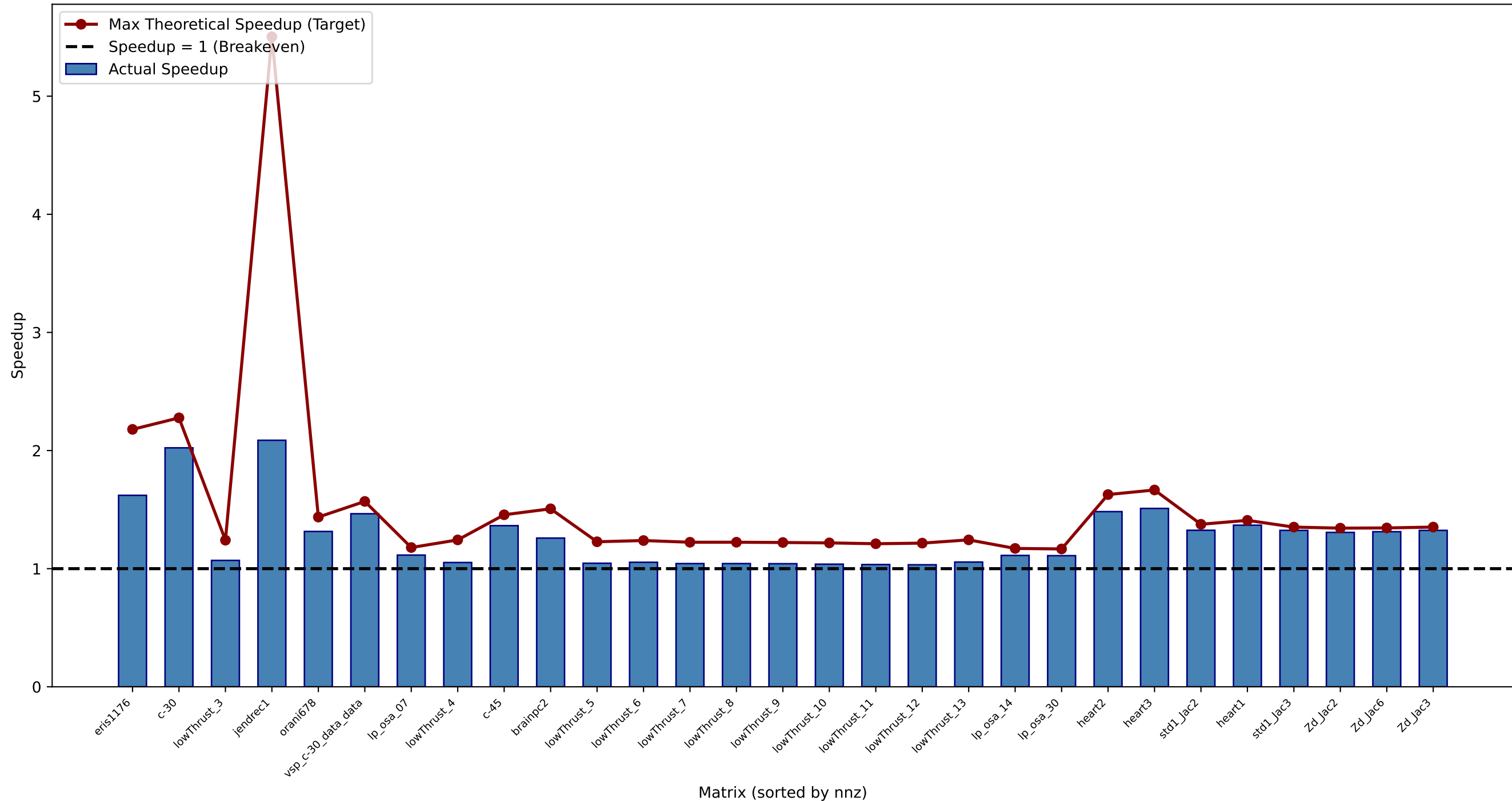
SpMM Speedups: dense=mkl, sparse=mkl (Line: Max Theoretical Target, Bars: Actual Achieved)
