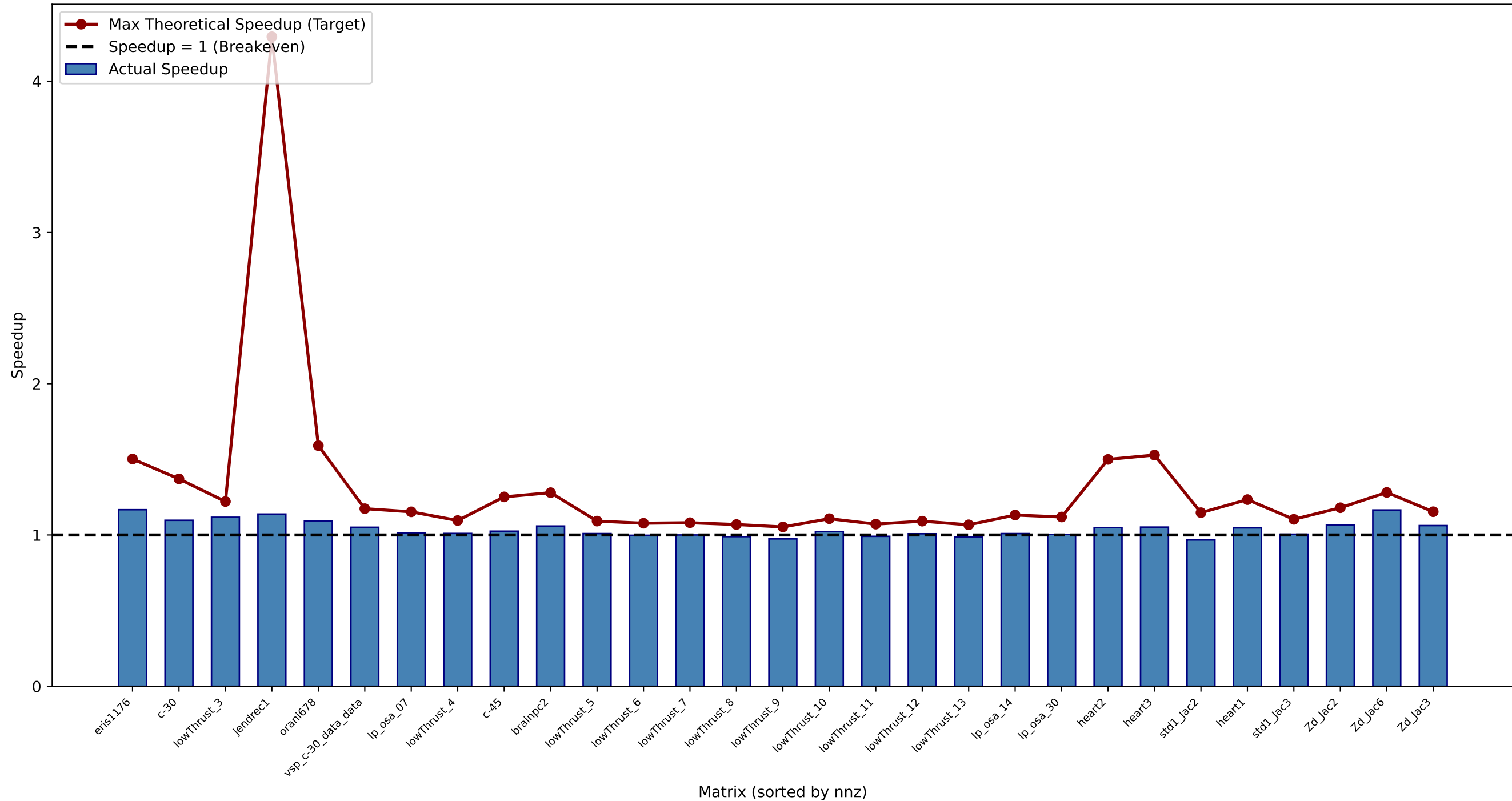
SpMV Speedups: dense=blas, sparse=naive (Line: Max Theoretical Target, Bars: Actual Achieved)
