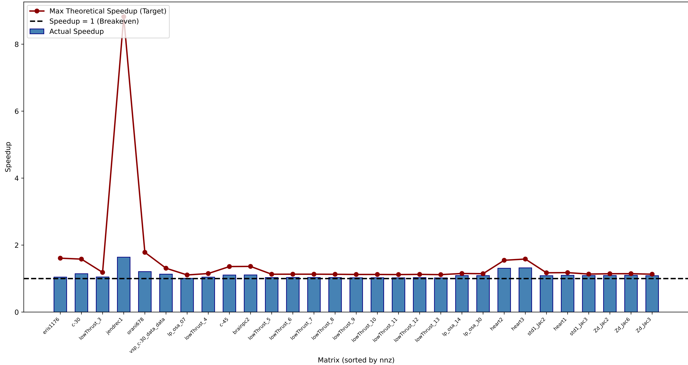
SpMV Speedups: dense=blas, sparse=spv8 (Line: Max Theoretical Target, Bars: Actual Achieved)
